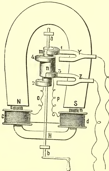
FIG. 31.—Stöhrer's commutator. For description see p. 49.
